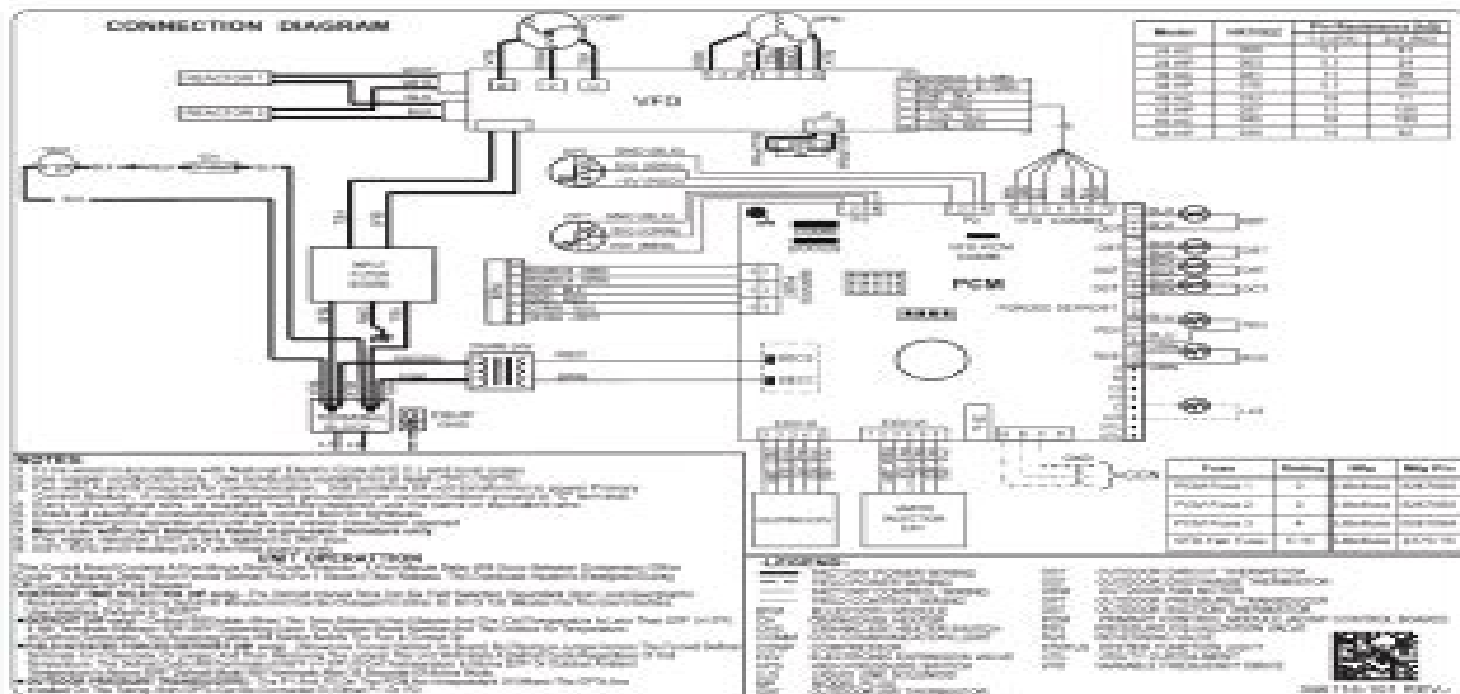
Fig. 1 – 186CNV024-50 Wiring Diagram
