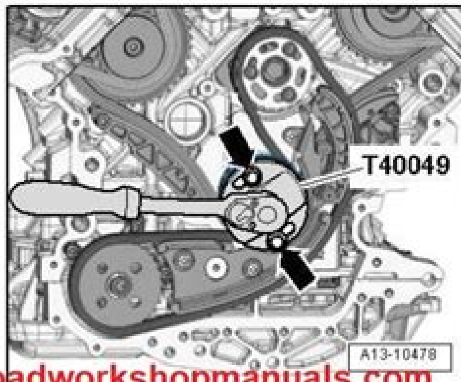
Fig. 142: Identifying Key T40049 At Rear On Crankshaft Installation
