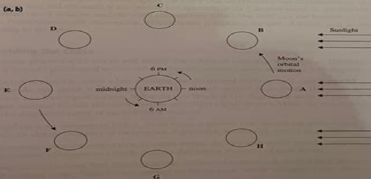
Figure 5-2 Top-down view of the Moon's orbit around Earth.
