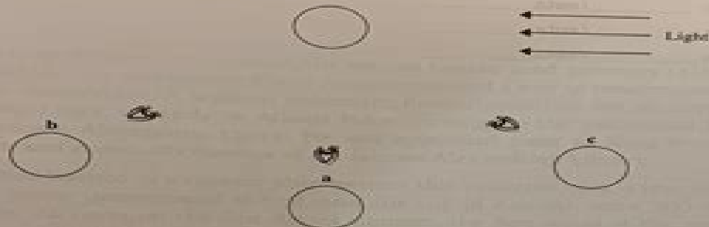
Figure 5-1 Phases of an illuminated ball.
