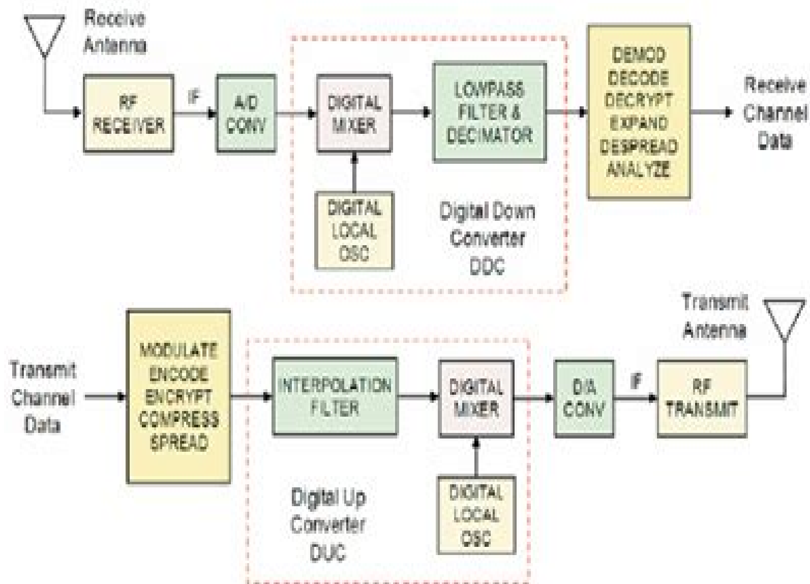
Figure 1. Signal-processing Blocks of a Typical Communications Transceiver System
