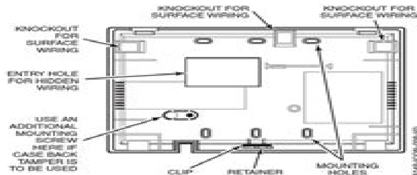
Figure 2. Mounting and Wiring Entry
