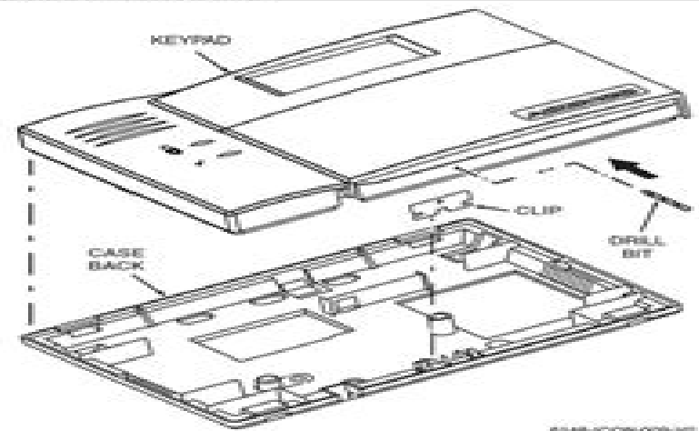
Figure 3. Locking Clip Installation (if required)
