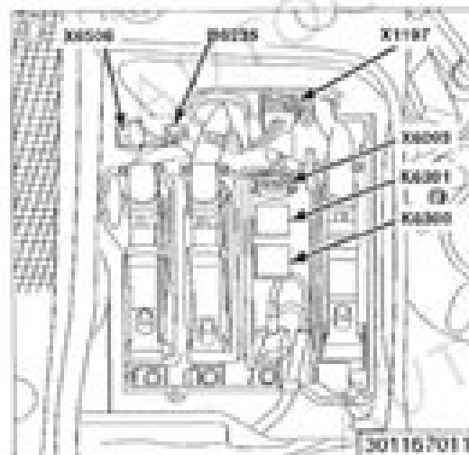
FIG. 2 - Rear RH side of engine compartment (S350)
