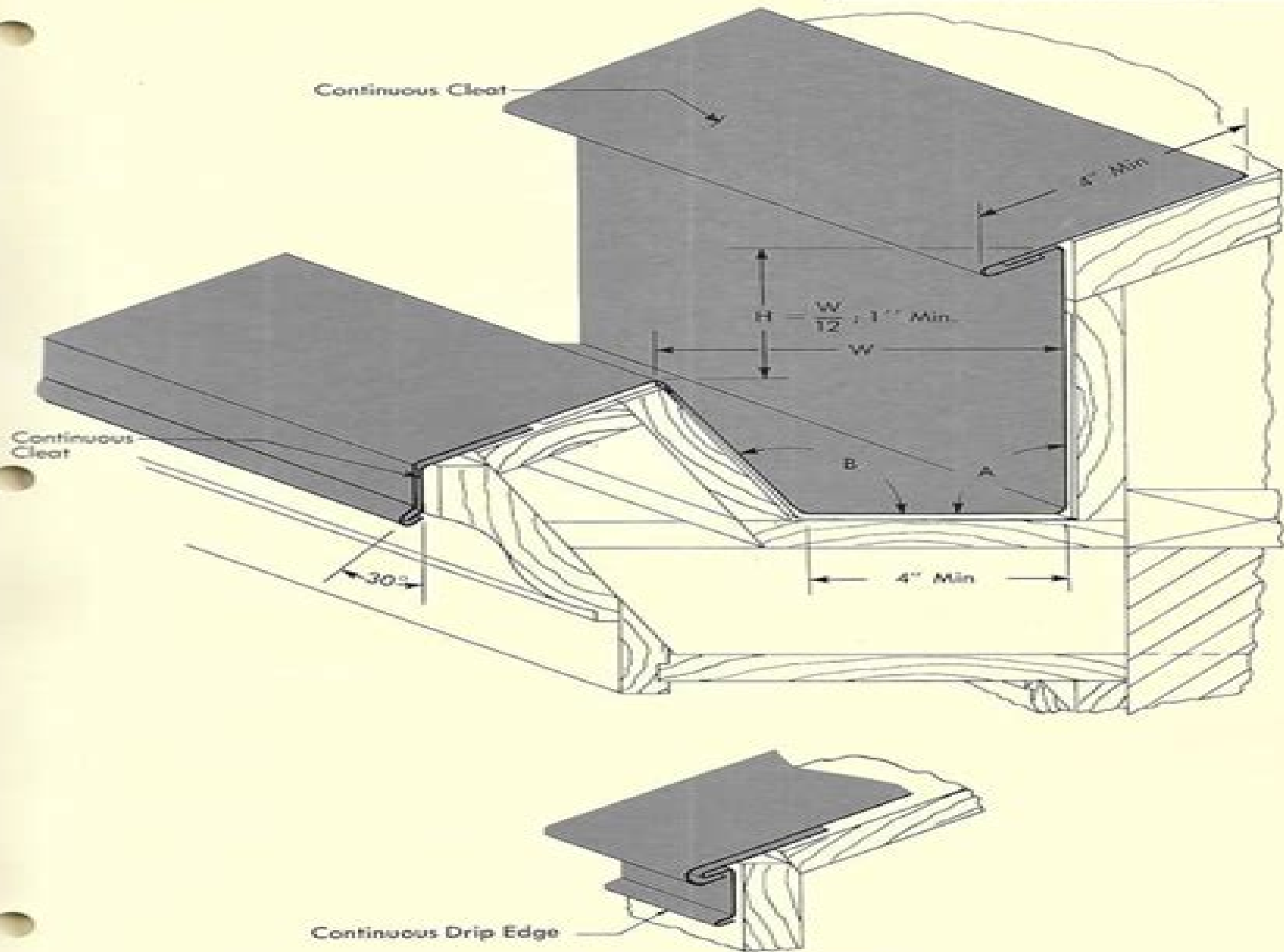
ALTERNATE DRIP EDGE DETAIL
