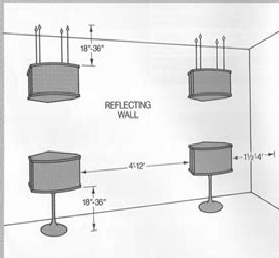
Figure 1. Recommended speaker placement in average-sized rooms.
