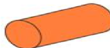
Cylinder
