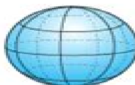
Sphere
