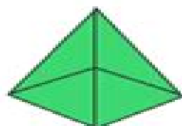
Square-based pyramid
