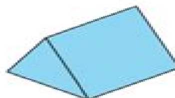
Triangular Prism
