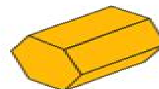
Hexagonal Prism
