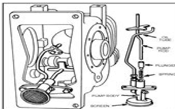
Fig. 562 – MODELS A, B OLD STYLE OIL PUMP
