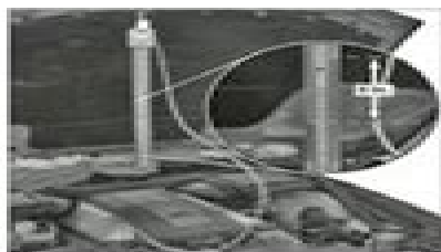
Use stick-tube manometer to diagnose defective crankcase breather valve, 130 Fuel Injection
