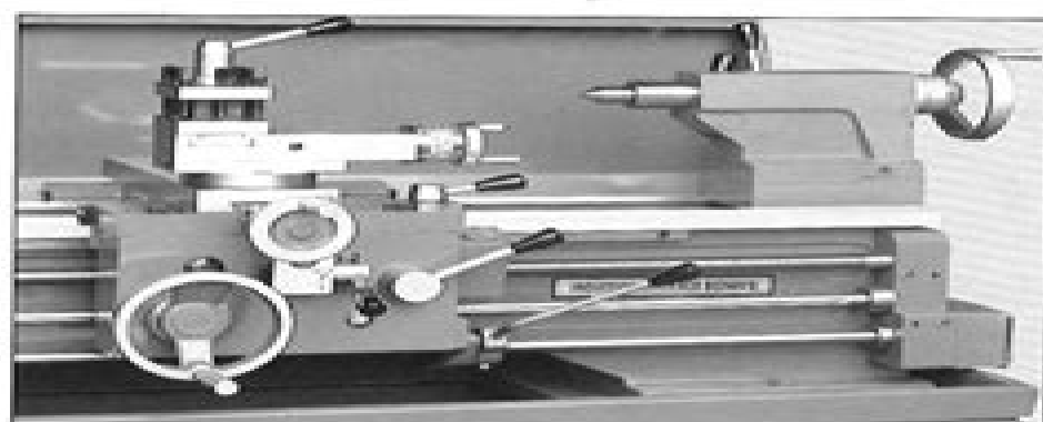
APRON & CARRIAGE
