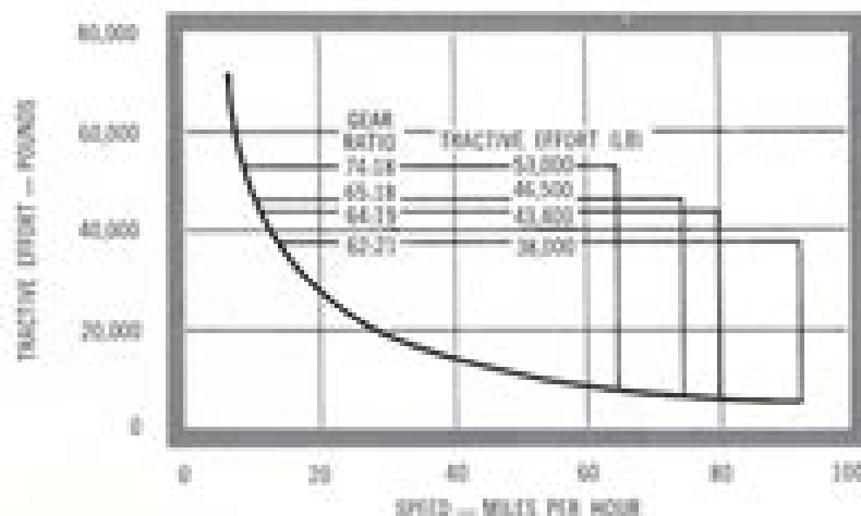
TRACTION EFFORT DL-212
