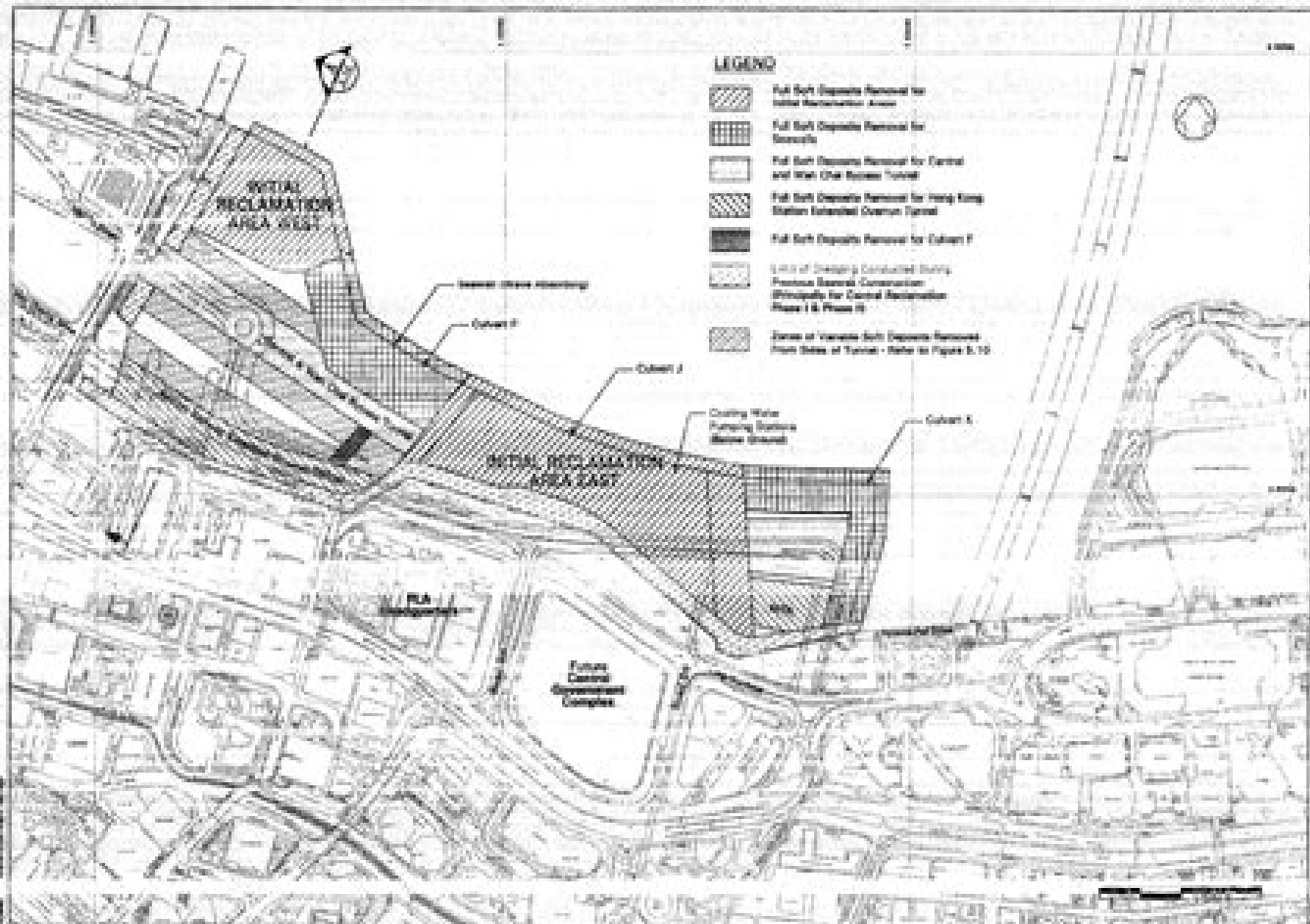
Recommended Reclamation Methods for Infrastructure Works
