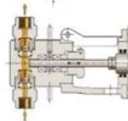
Packed plunger liquid end
