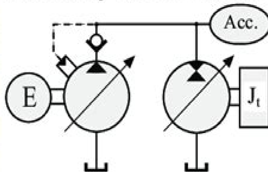
Secondary Motor Control
