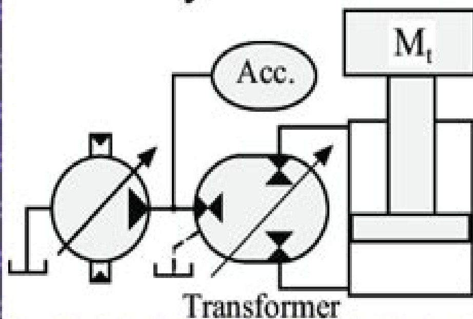
Secondary Trans Control
