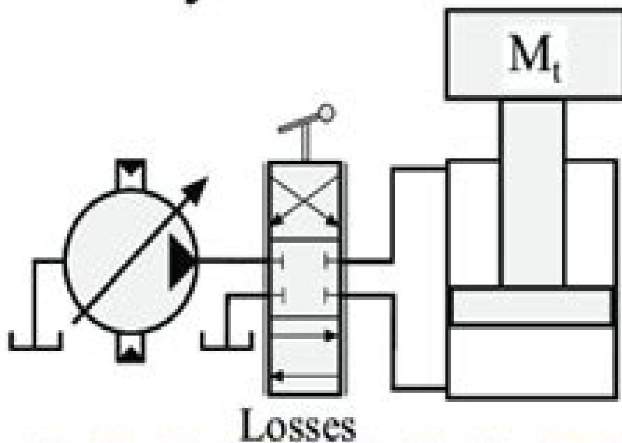
Primary Throttle Control
