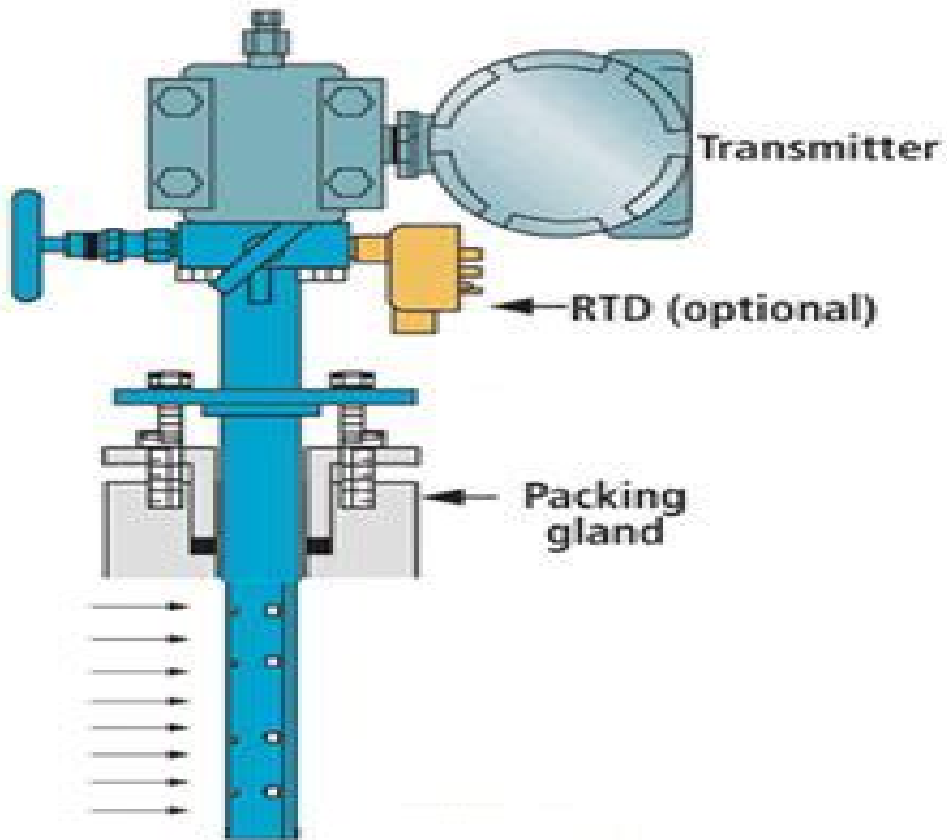
Annubar
