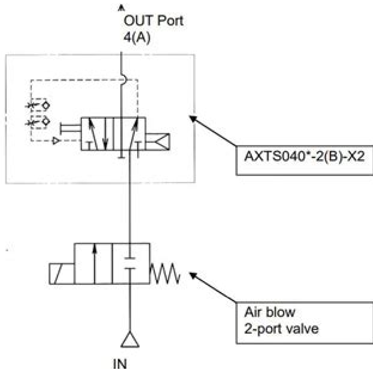
Fig.3 Symbol for internal pilot fluid passage.
