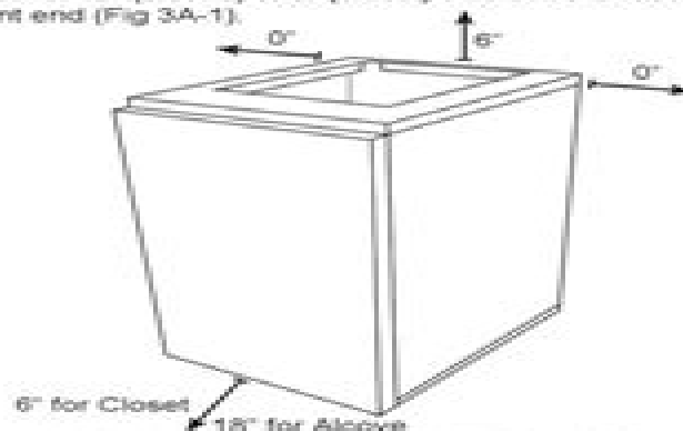
Fig 3A-1. Minimum Clearance for Electric Furnace
