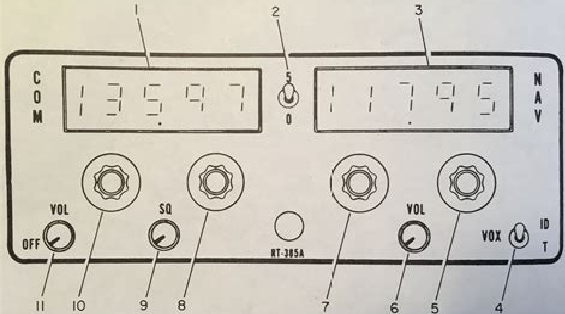
Figure 3-1. RT-385A Controls and Indicators.
