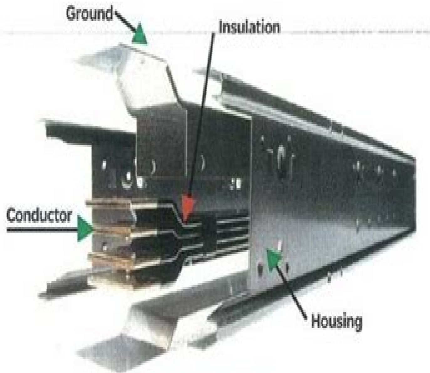
Fig.1 : Busway structure Fig 1: Busway structure
