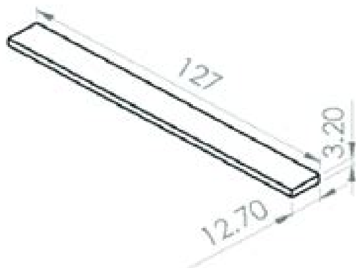
Flexural test specimen as per ASTM D790
