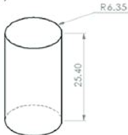
Compressive test specimen as per ASTM D695
