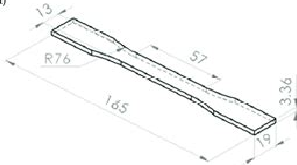
Tensile test specimen as per ASTM D638
