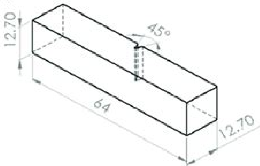
Izod Impact test specimen as per ASTM D256
