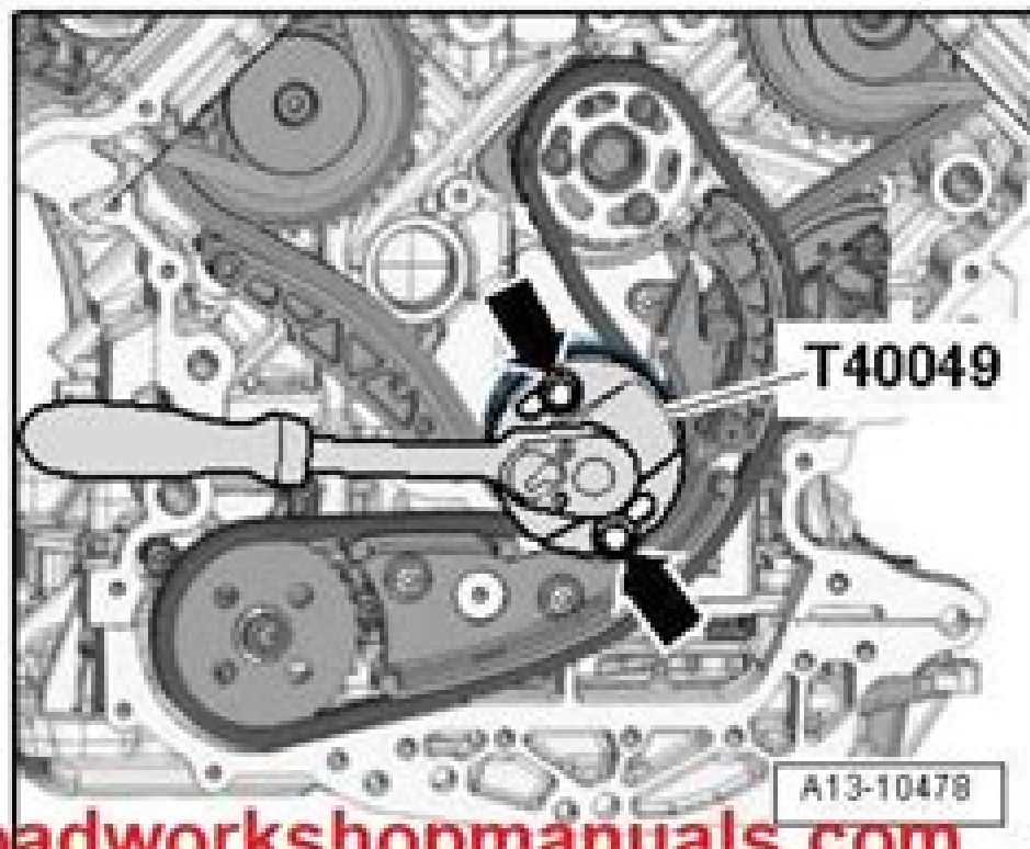
Fig. 142: Identifying Key T40049 At Rear On Cranksh. Installation
