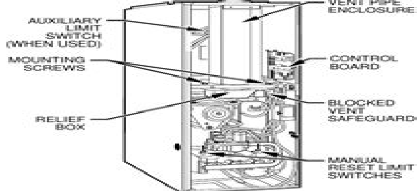
→ Fig. 7—Model 373LAV Downflow
