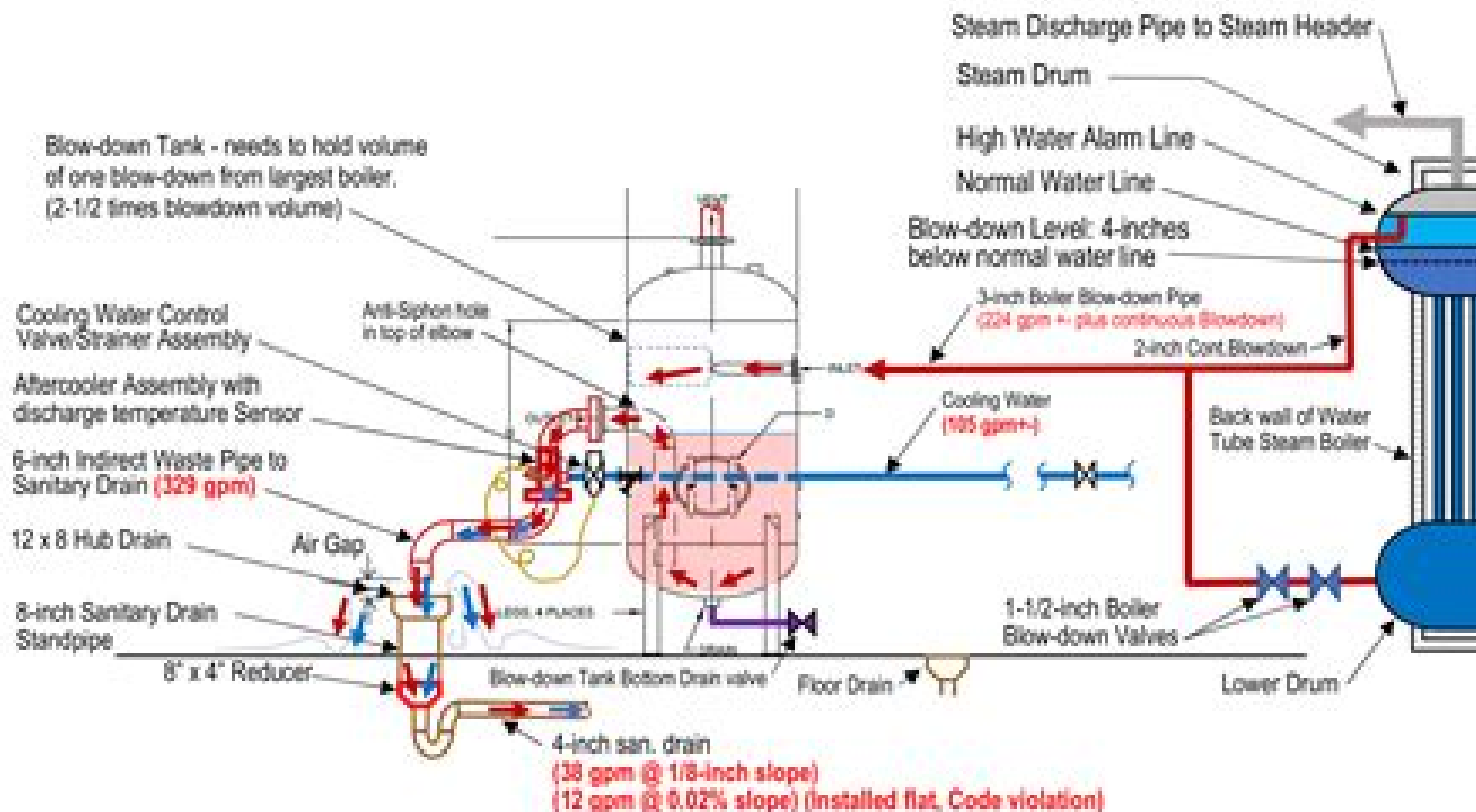
Figure 2: Boiler Blow-down Piping Diagram
