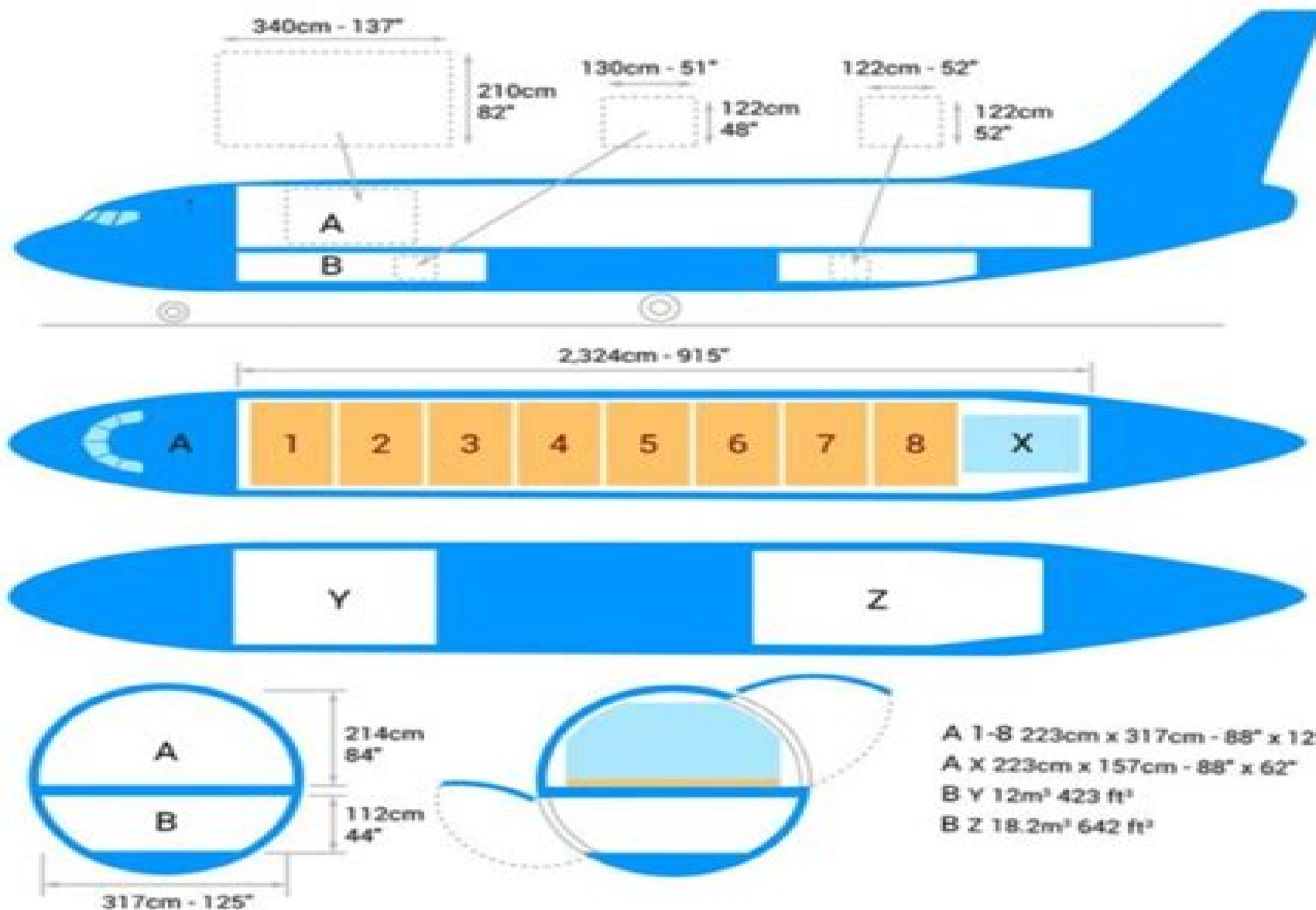
Boeing B737-300F
