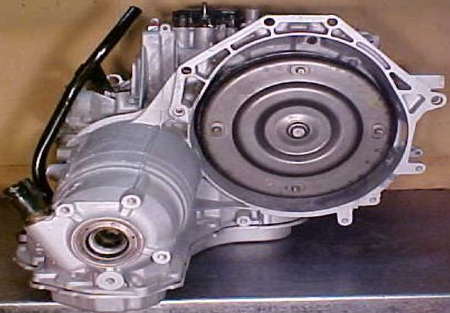
AX4N with torque converter installed.
