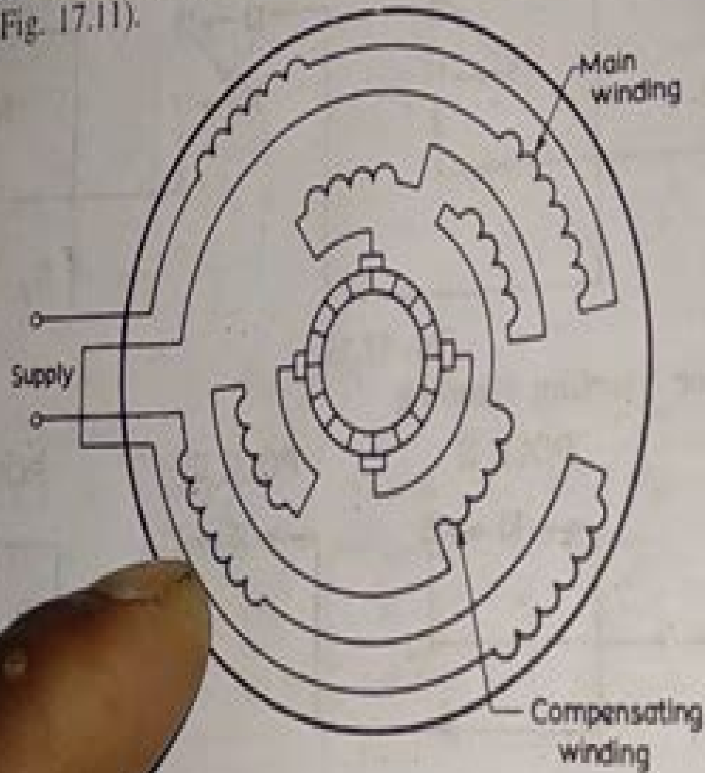
17.11. Use of compensating winding in repulsion motor.
