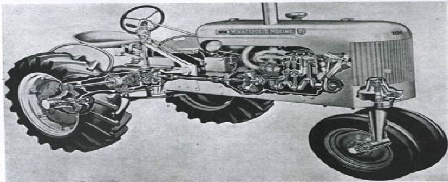
Minneapolis-Moline Model BF. Avery Models A and R were similarly constructed.
