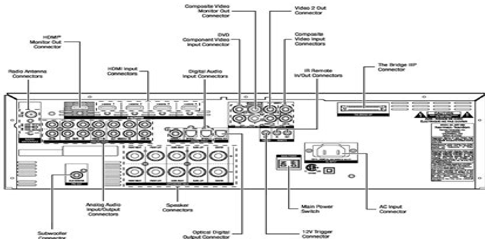
AVR 1650/AVR 165 Rear-Panel Connections (AVR 1650 shown)
