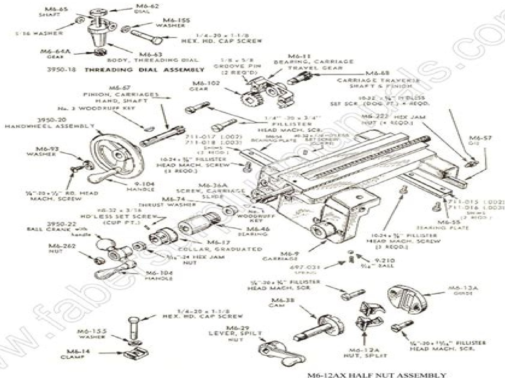
M6-9X CARRIAGE ASSEMBLY LESS COMPOUND REST AND THREADING DIAI
