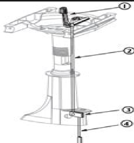
Figure 4 — Gear Selector Operation
