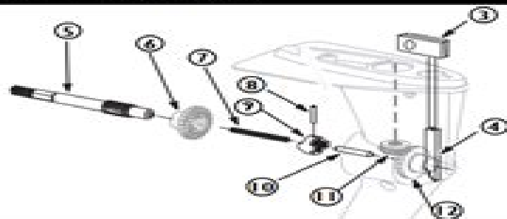
Figure 5 — Forward Gear
