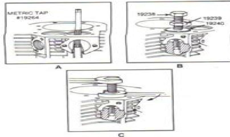
Fig. 10 - Pulling Brass or Sintered Iron Guide Bushing
