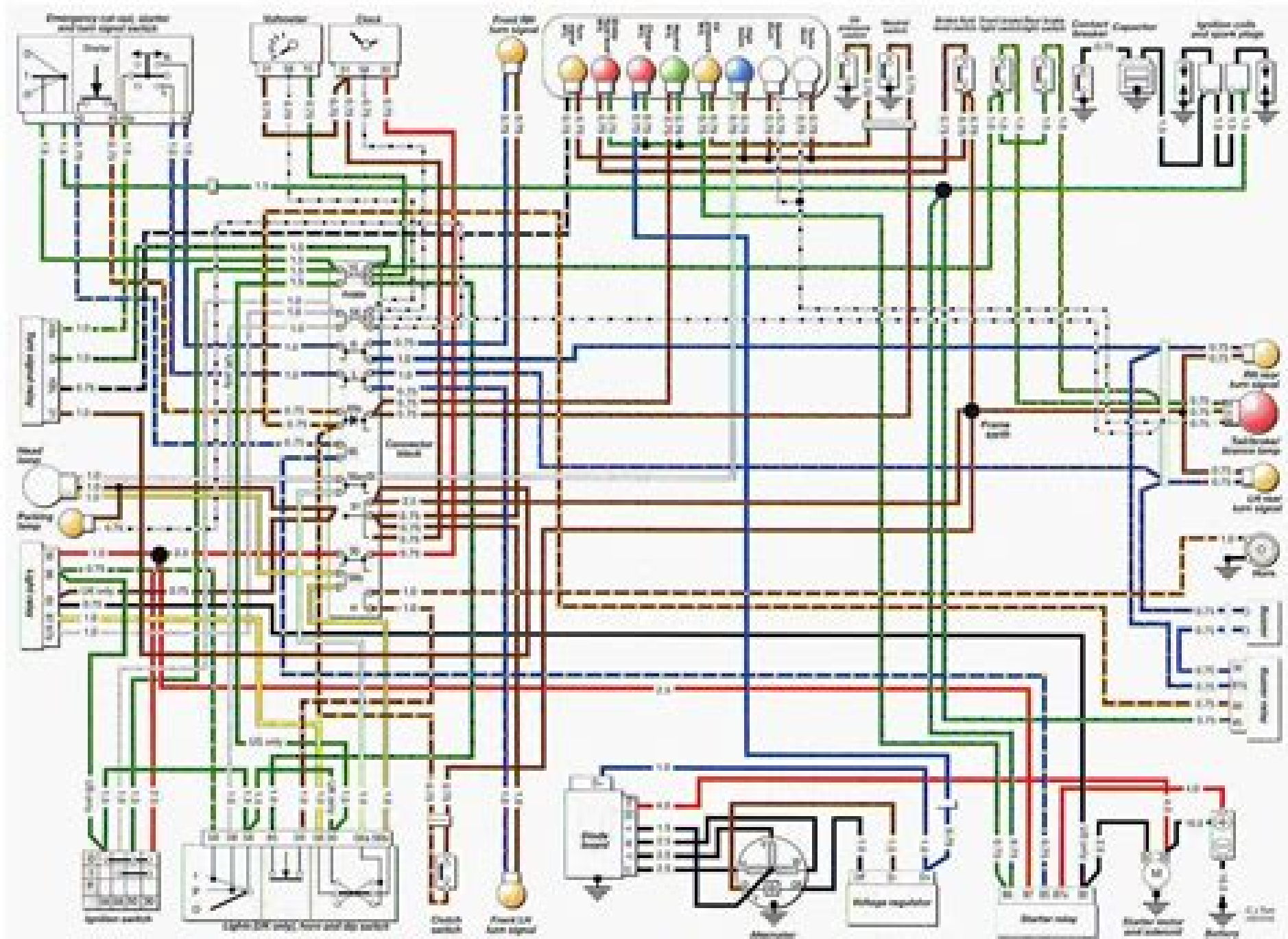
Wiring diagram - 1978 R60/T, R60/7, R100/T and R100S models
