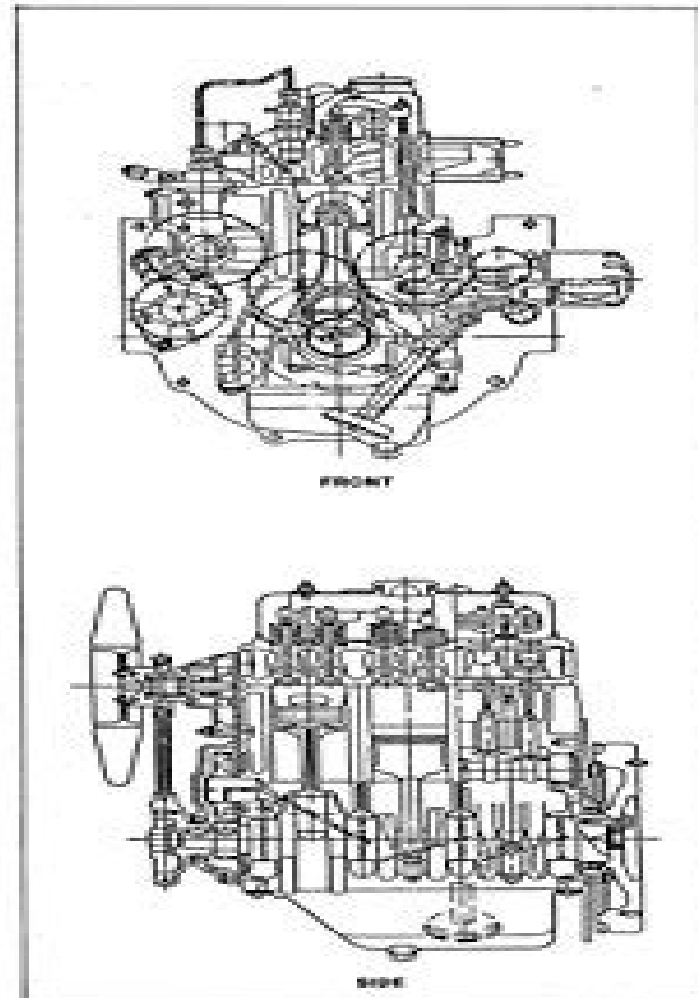
FIGURE 1 - CROSS SECTION VIEWS Side
