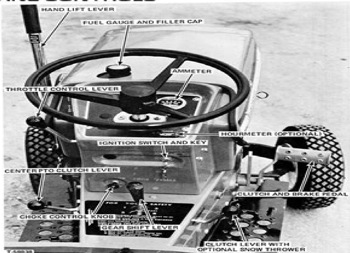
FIGURE 1 - Controls (Model 710 Standard 3 Speed Transmission Tractor)
