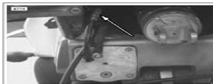
Figure 4-22. Fuel Pump Connector [86] (swingarm removed for illustration)
