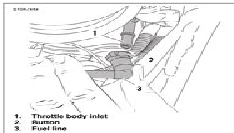
Figure 4-23. Fuel Line
