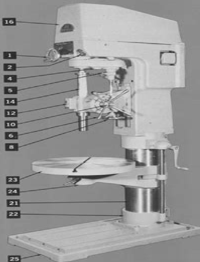
#3-B Round Column Type Floor Drill
