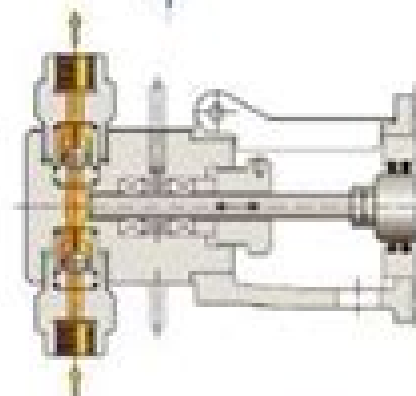
Packed plunger liquid end
