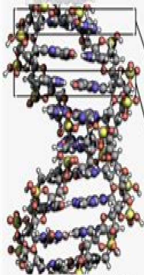
DNA
