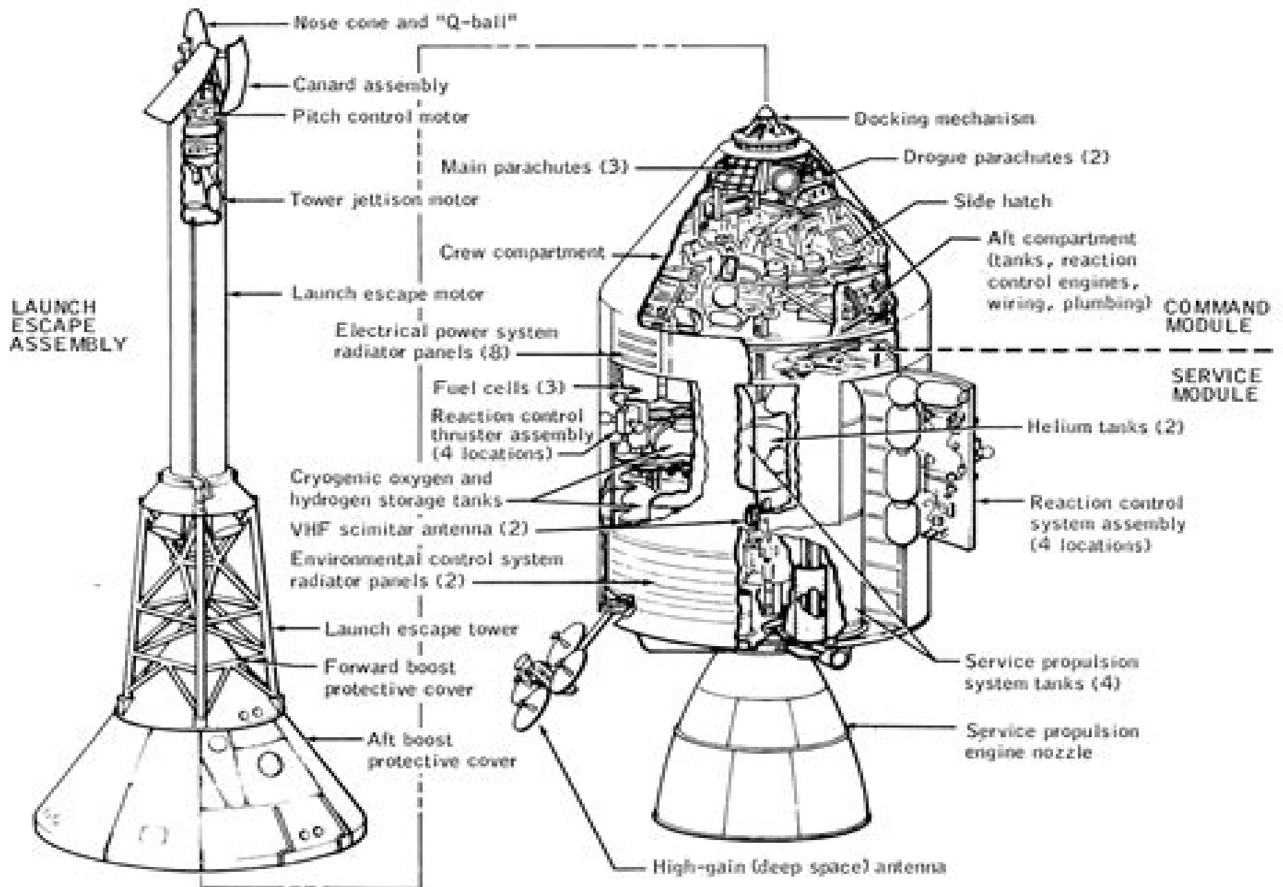
APOLLO COMMAND AND SERVICE MODULES AND LAUNCH ESCAPE SYSTEM
