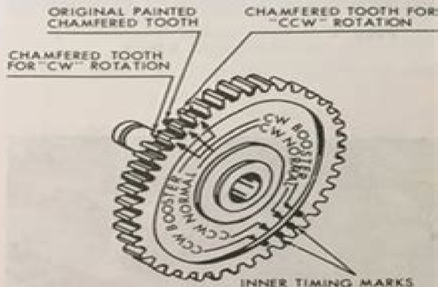
Figure 2-31. Six Cylinder Gear
