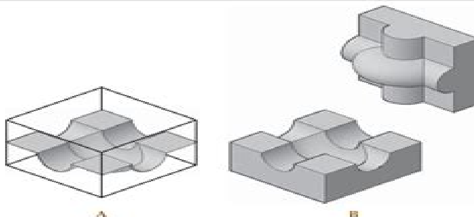
Figure 8-26. Slicing a solid with a surface. A —Draw the surface and locate it within the solid to be sliced. The solid is represented here by the wireframe. B —The completed slice with both sides retained. The top can now be moved and rotated as shown here.
