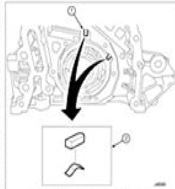
10.11b Fit the top oil pump side nut and side seal spring into the side of the timing cover.
