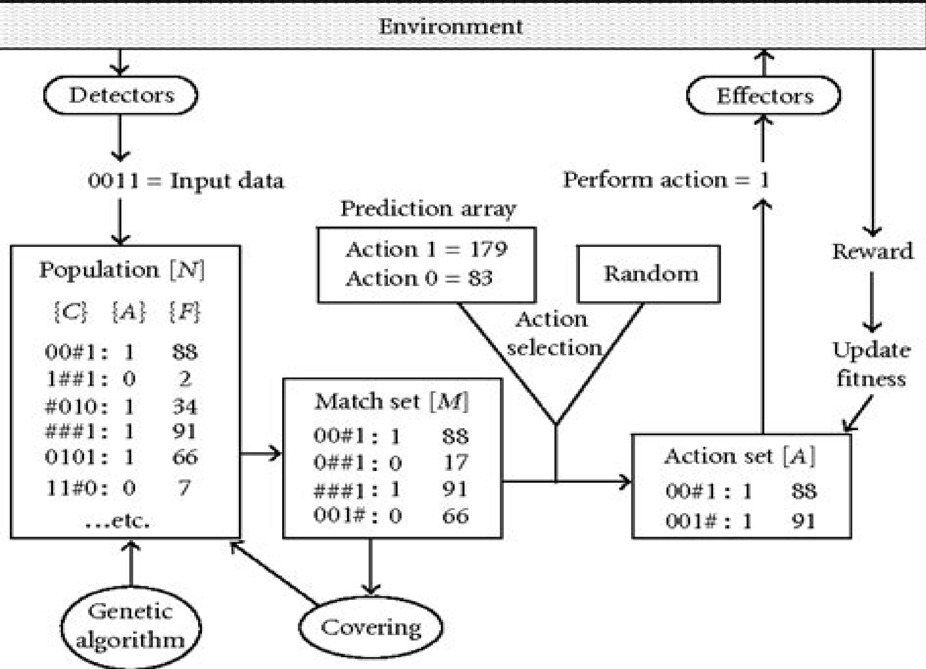
Figure 3: MCC algorithm for anomaly detection
