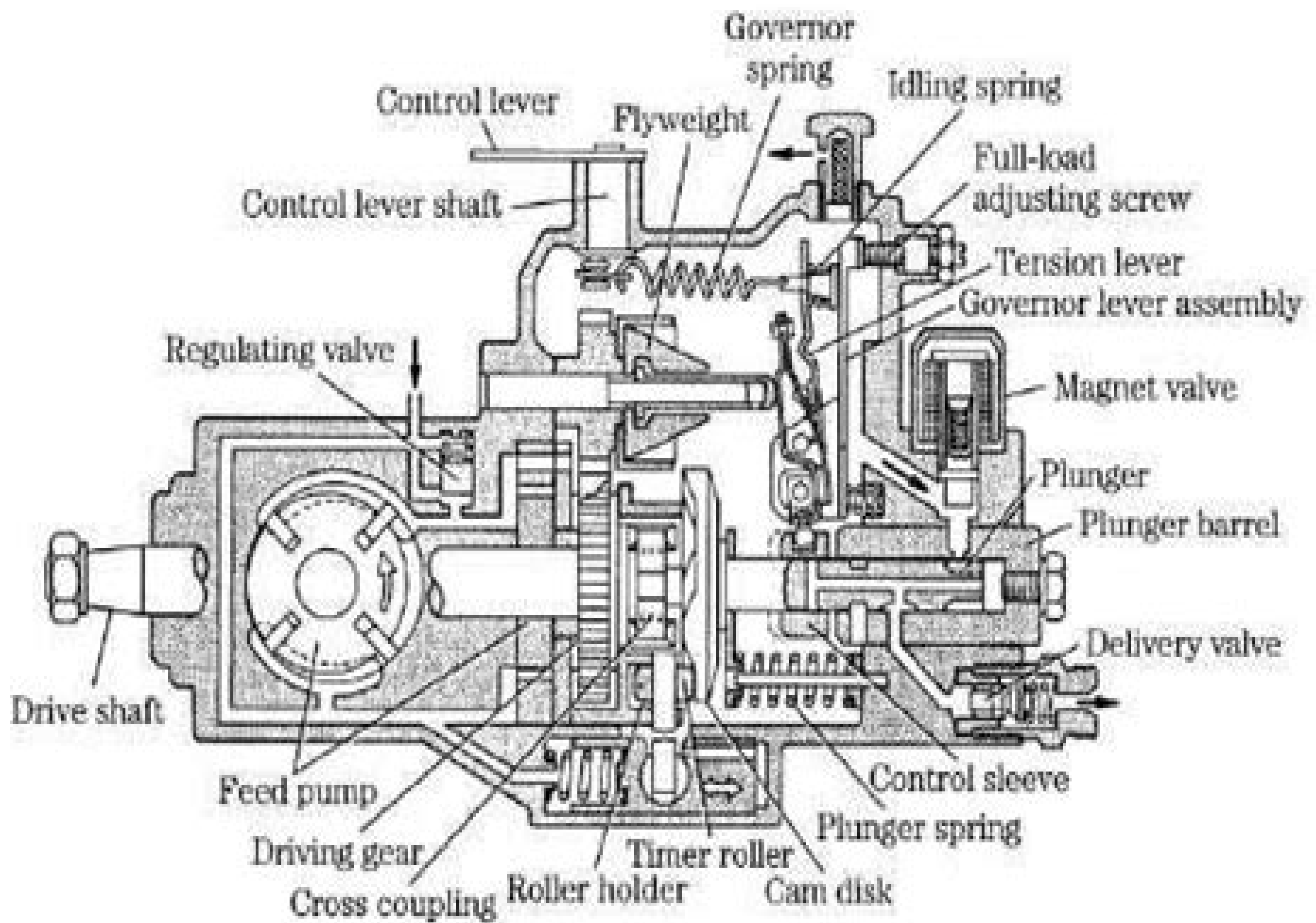
5-10 Bosch VE Series injection pump.
