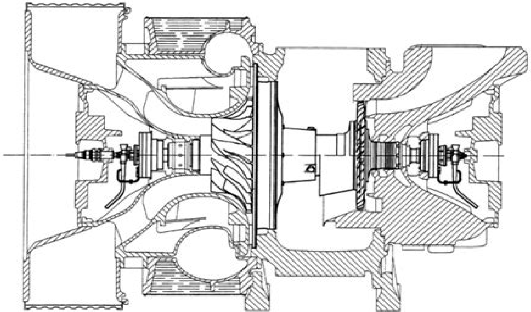
Turbocharger complete
