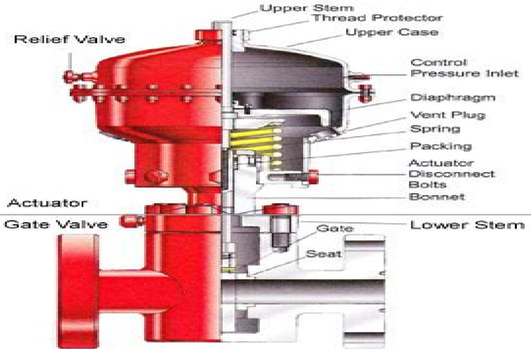
Actuator Mounted on a Reverse-Acting Gate Valve
