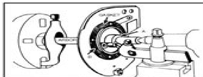
Fig. 892 – CORRECTING END PLAY
