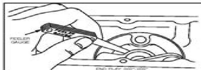
Fig. 893 – CHECKING CRANKSHAFT END PLAY
