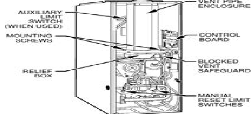
→ Fig. 7—Model 373LAV Downflow
